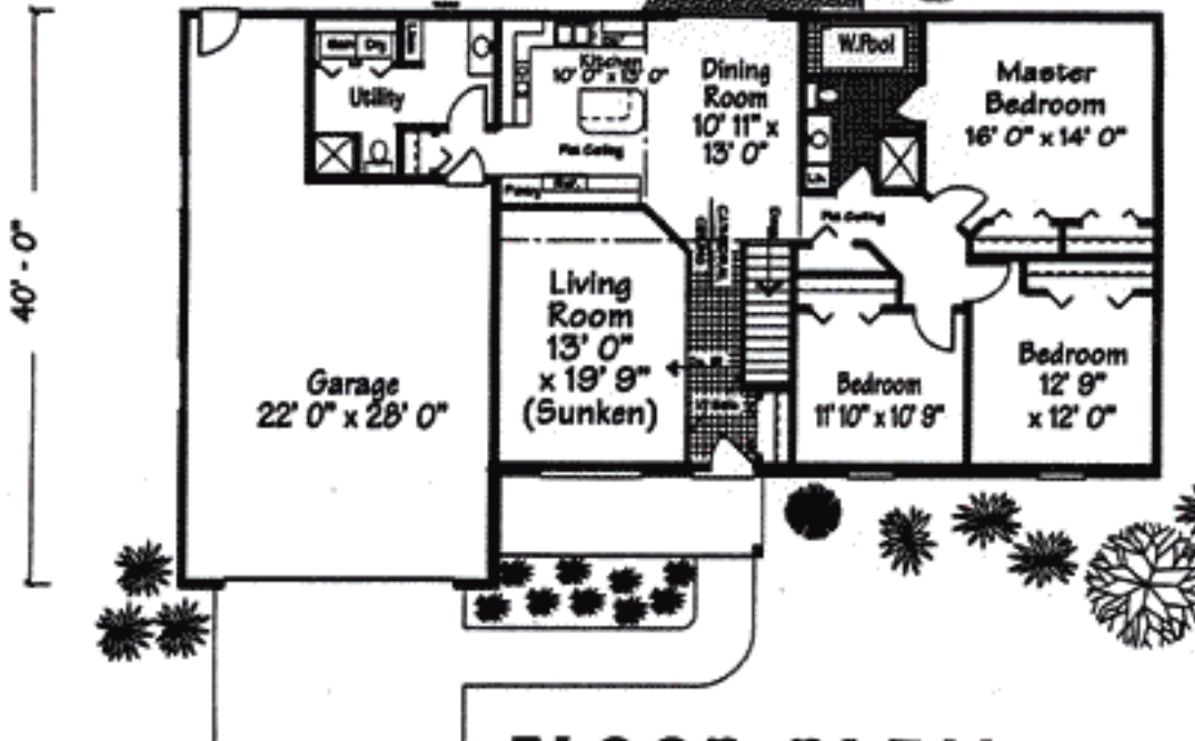
FLOOR PLAN 1660 Sq. Ft.
