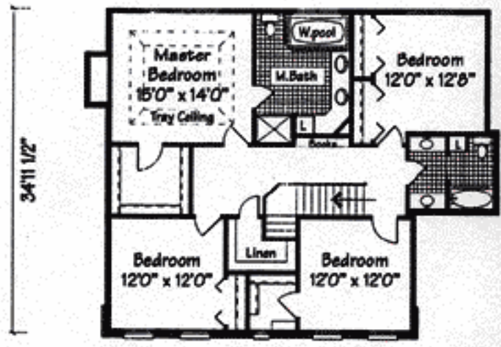
SECOND FLOOR PLAN 1298 Sq. Ft.
