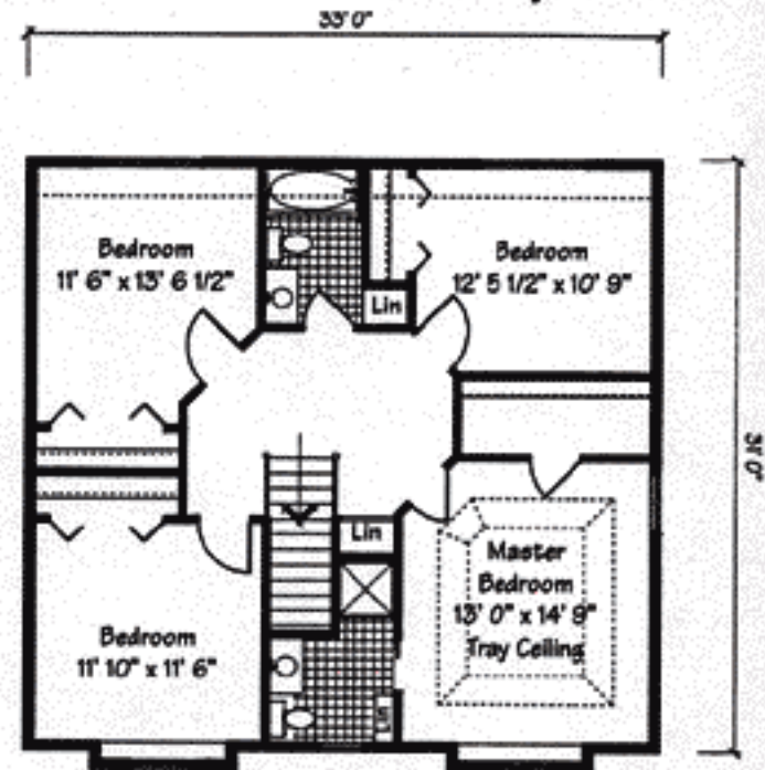
SECOND FLOOR PLAN 993 Sq. Ft.
